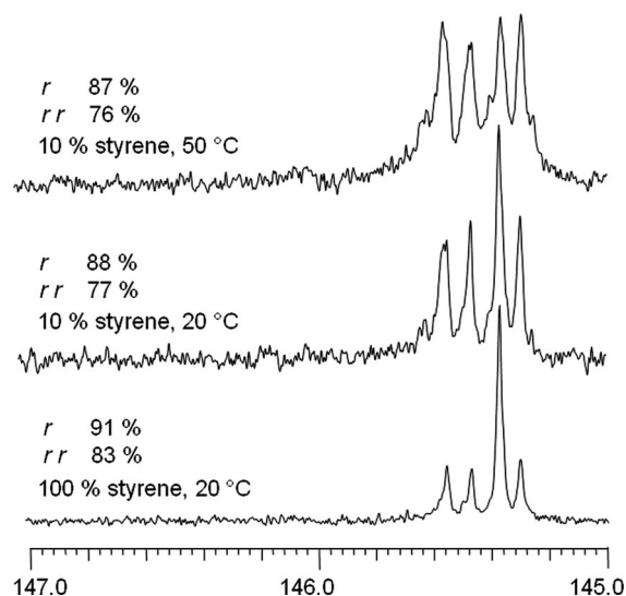
Figure 5. ^{13}\text{C} NMR signals of the phenyl \text{C}_{\text{ipso}} atom in the polystyrene materials ( [\text{D}_2] tetrachloroethane, T = 100\text{ }^\circ\text{C} ) obtained with initiator 5 under various conditions.
