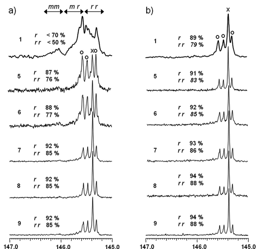
Figure 4. ^{13}\text{C} NMR signals of the phenyl \text{C}_{\text{ipso}} atom in the polystyrene materials ( [\text{D}_2] tetrachloroethane, T = 100\text{ }^\circ\text{C} ). a) Polymers obtained with the various initiators 1, 5–9; 10% styrene solutions in cyclohexane; 50 °C. b) Polymers obtained with the various initiators 1, 5–9; 100% styrene; 20 °C. The syndiotactic rrrrrr heptade is marked by \times , and the error heptades mr , rrr and rrrr by \circ .
