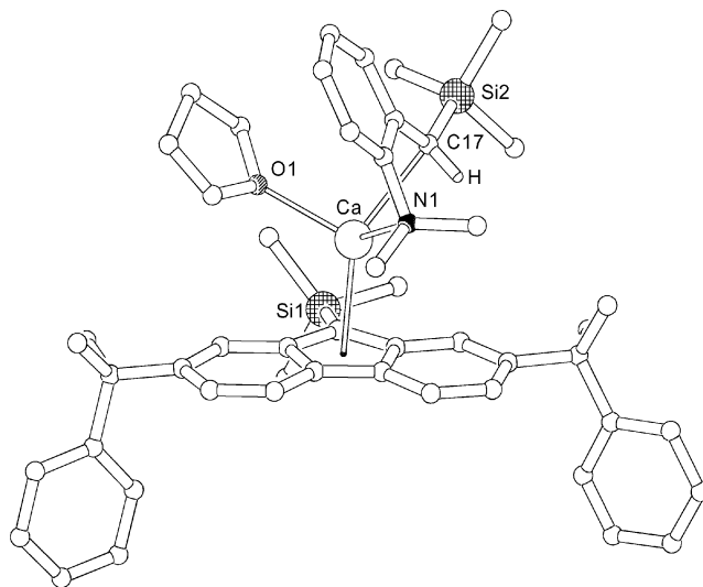
Figure 3. Crystal structure of 6 . Except for the benzylic hydrogen, all hydrogen atoms have been omitted for clarity. Selected bond lengths [Å] and angles [°]: Ca–C17 2.517(3), Ca–N1 2.496(2), Ca–O1 2.331(2); Ca–C(fluorenyl): 2.631(2), 2.647(2), 2.768(2), 2.779(2), 2.843(2); C17–Ca–N1 70.95(8), C17–Ca–O1 99.63(8), N1–Ca–O1 113.37(6).
