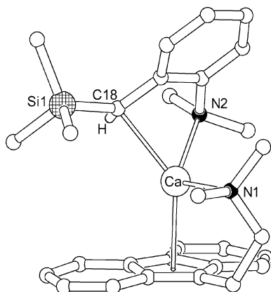
Figure 1. Crystal structure of 4 . Only one of the two crystallographically independent, but very similar, molecules is shown. Except for the benzylic hydrogen, all hydrogen atoms have been omitted for clarity. Average selected bond lengths [Å] and angles [°]: Ca–C18 2.508(3), Ca–N1 2.487(2), Ca–N2 2.460(2); Ca–C(fluorenyl): 2.630(3), 2.658(3), 2.727(3), 2.739(3), 2.782(3); C18–Ca–N1 113.6(1), C18–Ca–N2 71.4(1), N1–Ca–N2 112.0(1).
