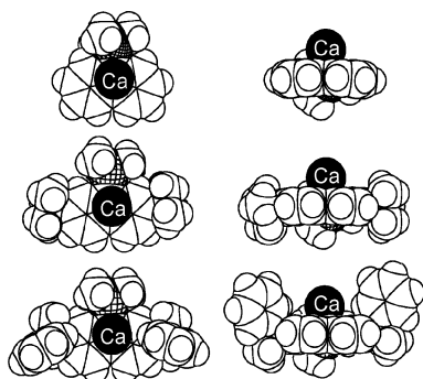
Figure 6. Space-filling models of the fluorenyl–Ca unit with increasing steric bulk of the fluorenyl ligand (top to bottom) as in the initiators 1 , 5 and 6 . Left: view perpendicular to the fluorenyl plane. Right: view along the fluorenyl plane.
