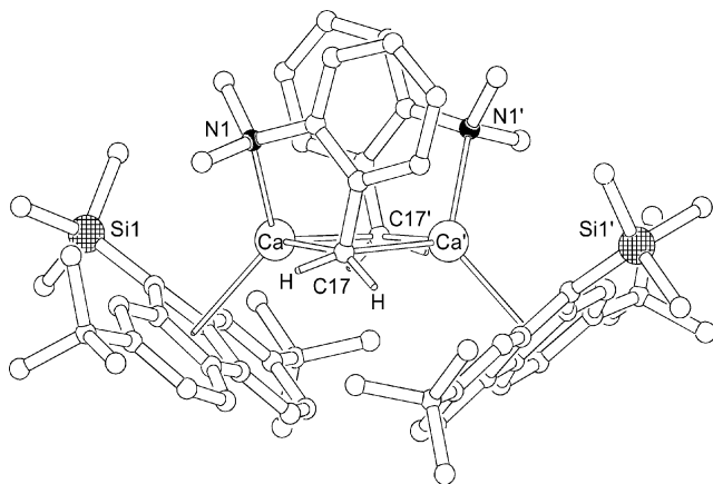
Figure 2. Crystal structure of 5 . Except for the benzylic hydrogen atoms, all hydrogen atoms have been omitted for clarity. Selected bond lengths [Å] and angles [°]: Ca–C17 2.572(2), Ca–C17' 2.572(2), Ca–N1 2.568(2); Ca–C(fluorenyl): 2.698(2), 2.705(2), 2.749(2), 2.796(2), 2.800(2); Ca...Ca' 3.5074(6), C17–Ca–C17' 93.95(6), C17–Ca–N1 68.08(5), C17'–Ca–N1 120.08(5).
